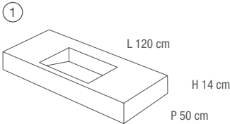
DAVE WASHBASIN FRONT FALL L-SHAPE WITH SINK 52,5x31x4-10H cm
