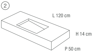
DAVE WASHBASIN SIDE FALL L-SHAPE WITH SINK 51x32,5x4-10 cm
